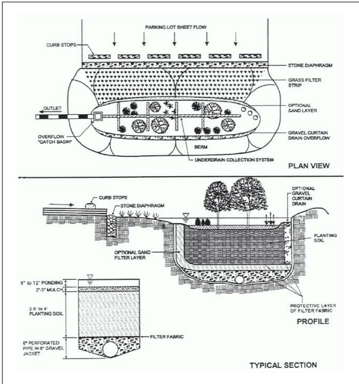
Figure 5: Bioretention system
