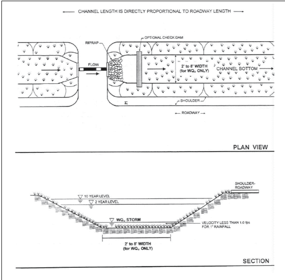
Figure 1: Grass swale
