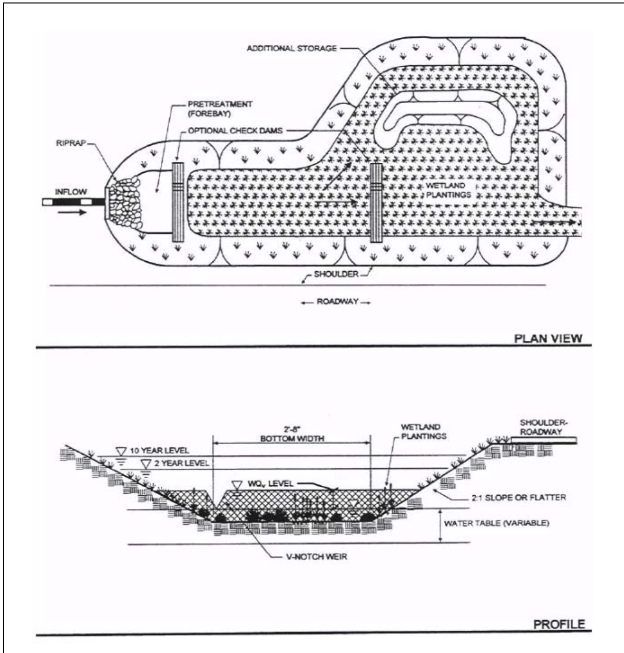
Figure 3: Wet swale
