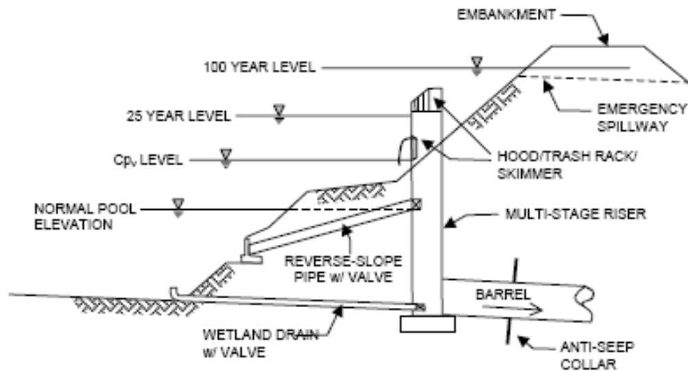
Figure 7: Typical wetland facility outlet structure
