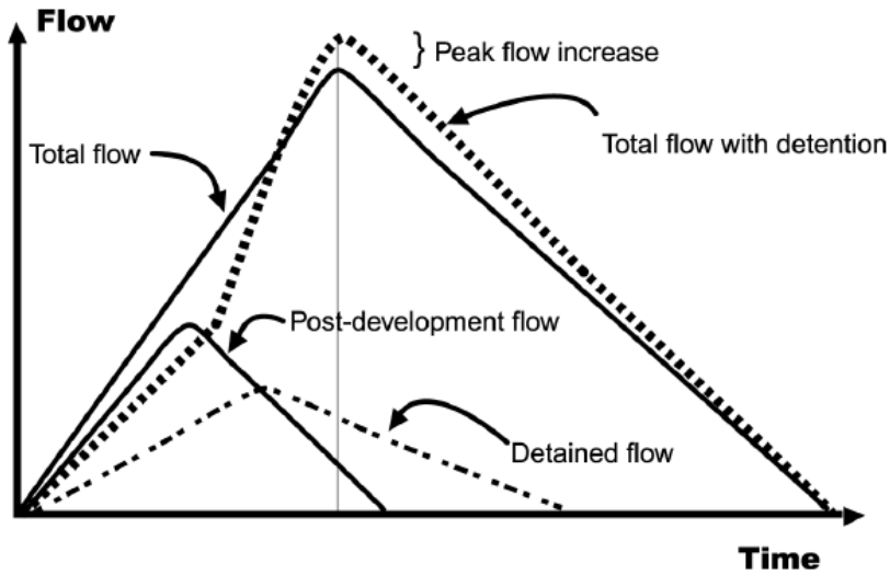
Figure 1: Example of detention timing
