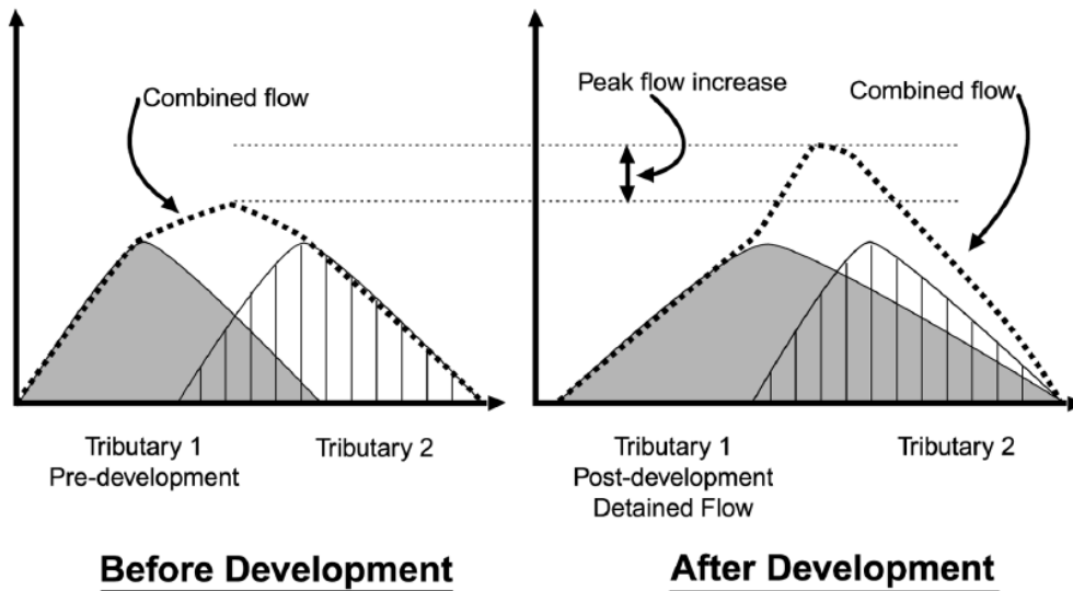
Figure 2: Impact of increased post-development volume with detention on a downstream hydrograph
