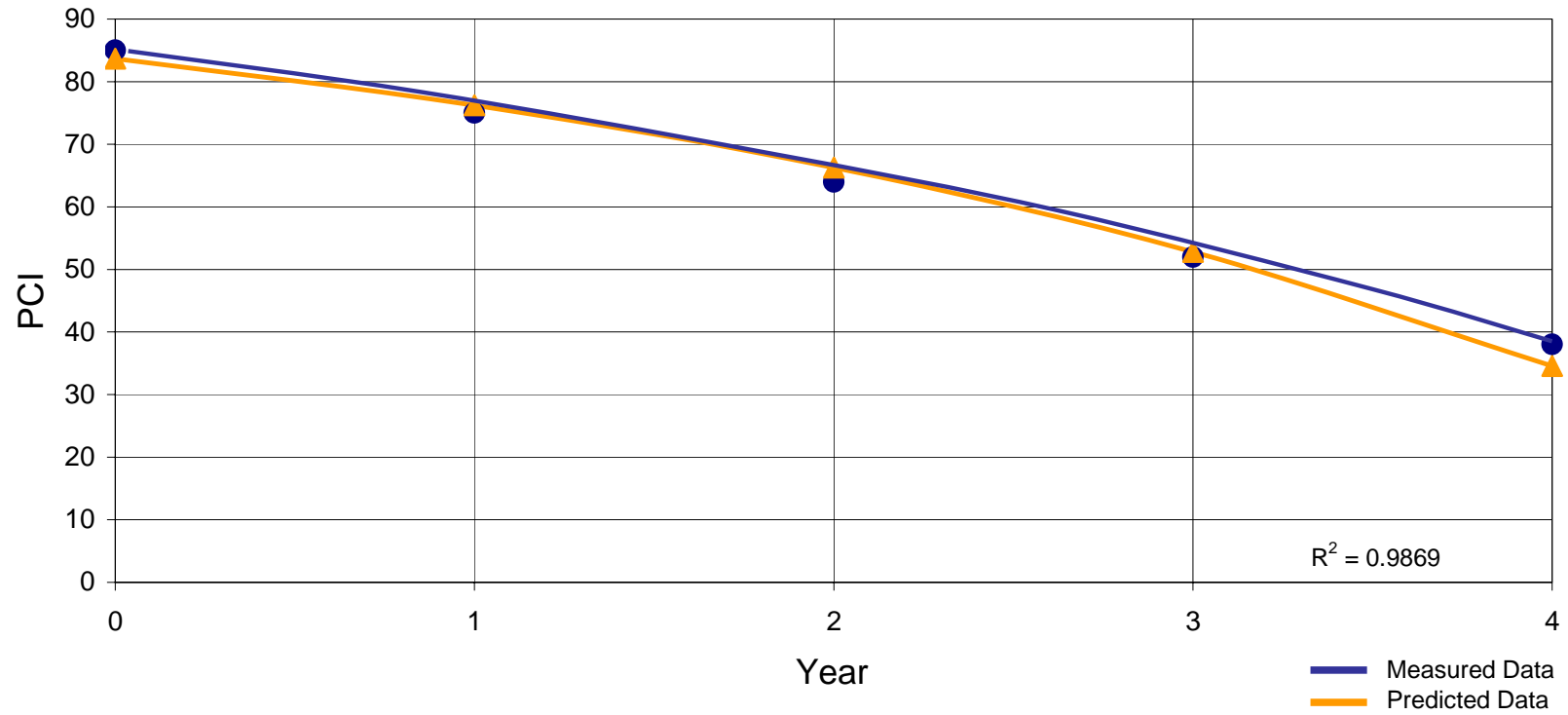
Slurry Seal - Flexible Pavement (Poor Condition, ADT > 5000, Trucks > 5%)
