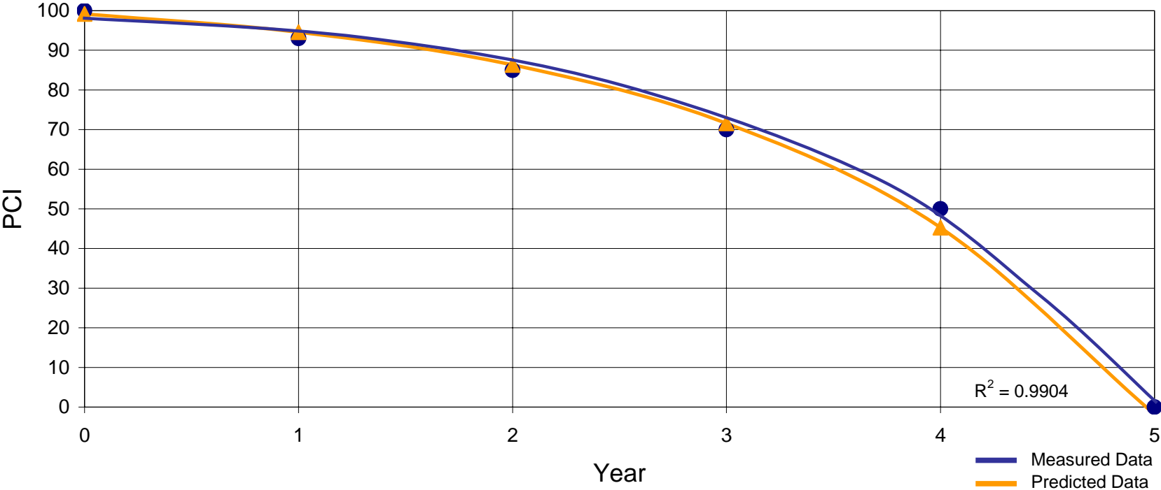
8" Base Stabilization Plus Double Chip Seal
