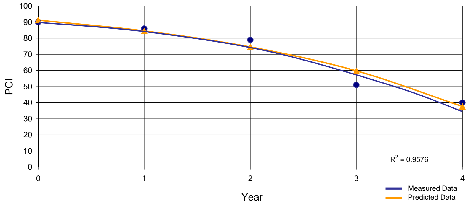
Slurry Seal - Flexible Pavement (Fair Condition, ADT > 5000, Trucks > 5%)
