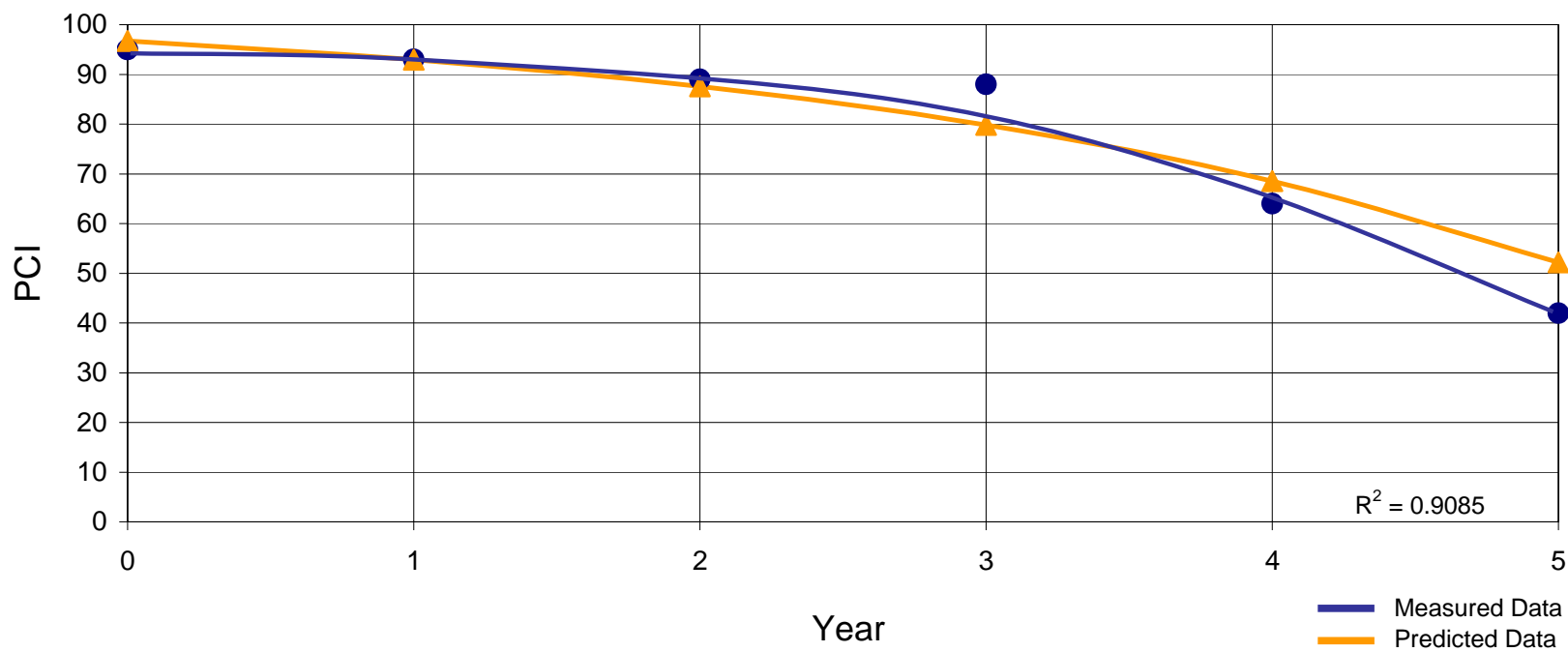
Slurry Seal - Flexible Pavement (Fair Condition, ADT < 5000, Trucks < 5%)
