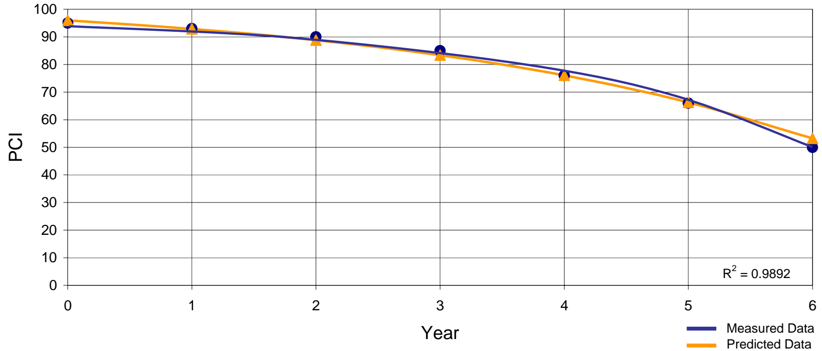
8" Stabilized Base Plus 2" A.C. Overlay
