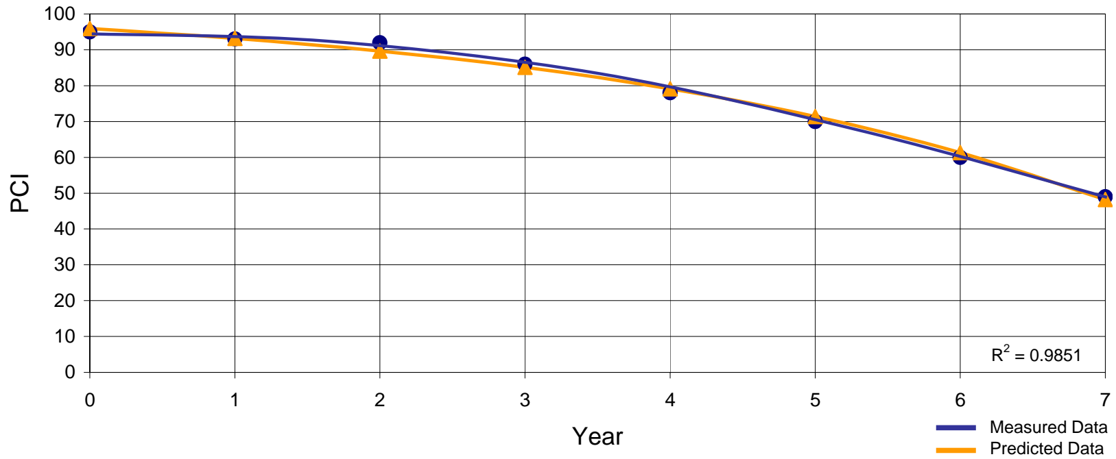
4" A.C. Overlay - Flexible Pavement (Poor Condition, ADT < 5000, Trucks < 5%)
