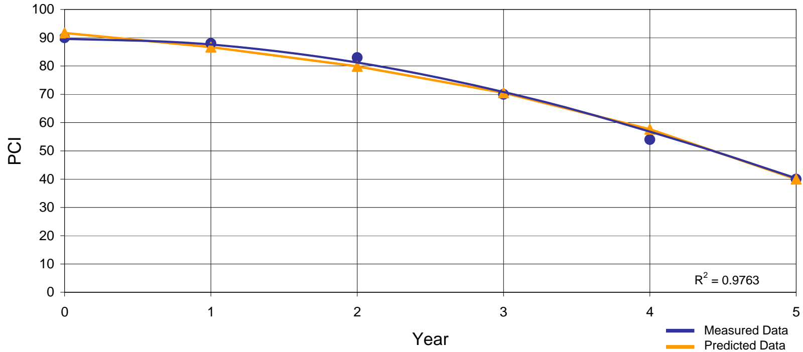
2" A.C. Overlay - Flexible Pavement (Poor Condition, ADT < 5000, Trucks < 5%)
