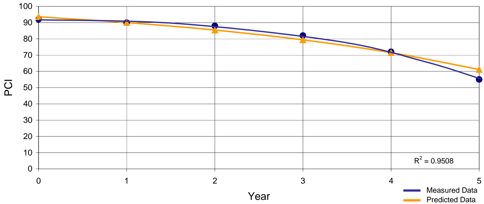
4" A.C. Overlay - Flexible Pavement (Poor Condition, ADT > 5000, Trucks > 5%)
