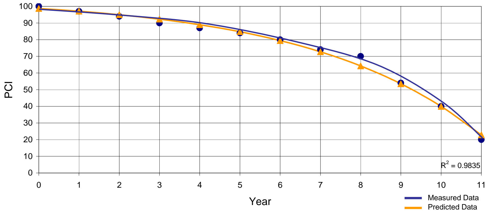
8" Stabilized Base Plus 4" A.C. Overlay
