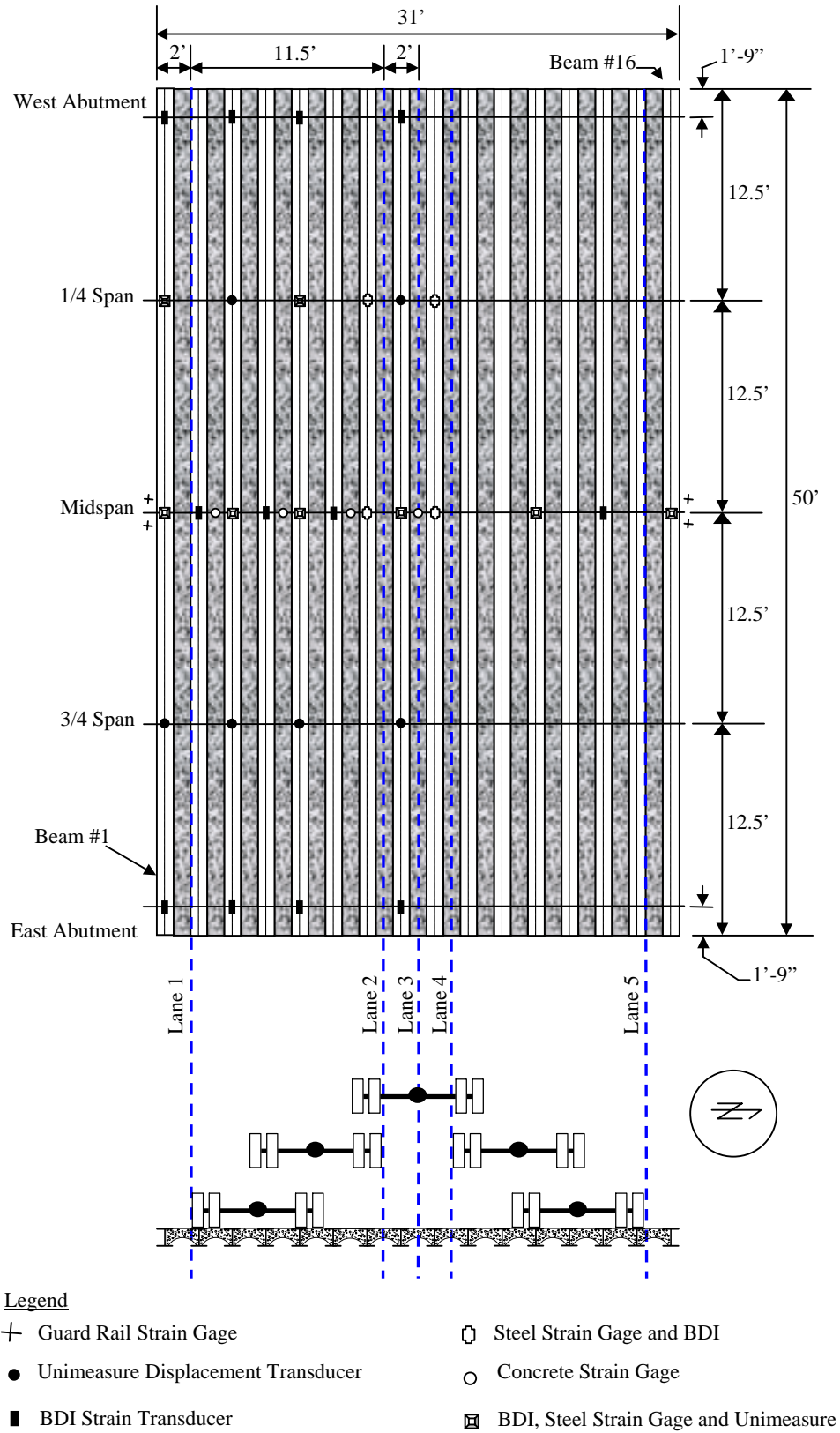
FIGURE 5 Layout of Instrumentation and Location of Lanes
