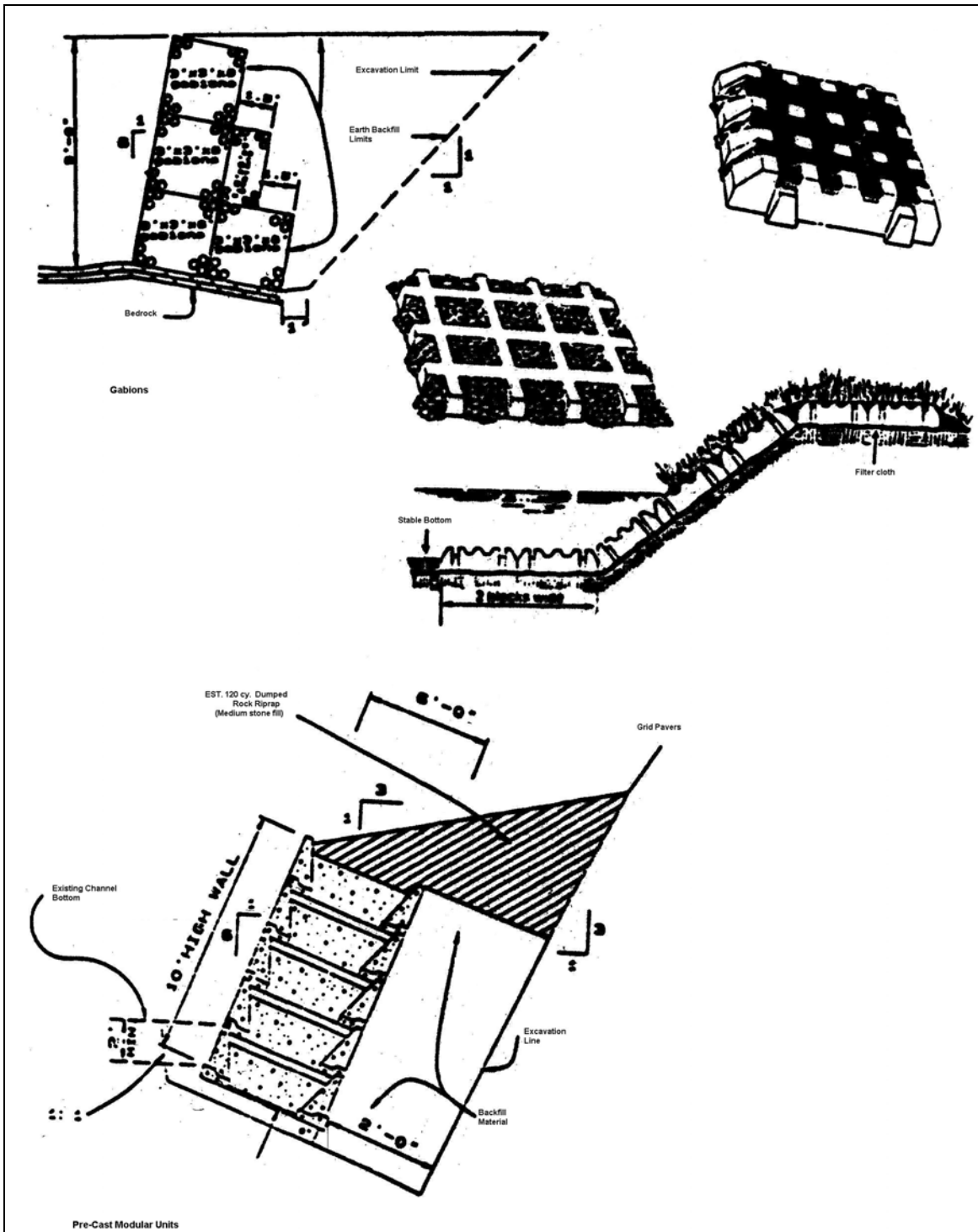
Figure 3.32. Streambank protection measures (Source: Department of Civil, Construction, and Environmental Engineering, Iowa State University)
