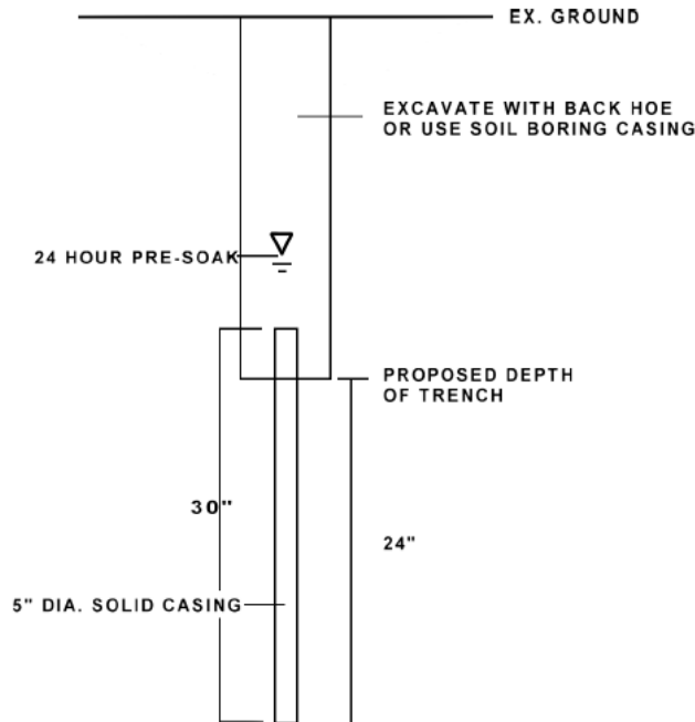
Figure 1: Infiltration testing requirements
