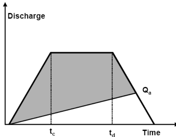
Figure 4: Modified Rational hydrograph definitions
