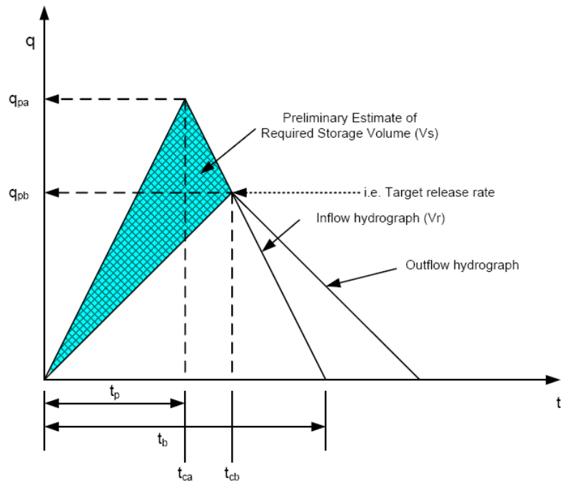
Figure 3: General schematic for estimating the volume of required storage (cross-hatched area)
