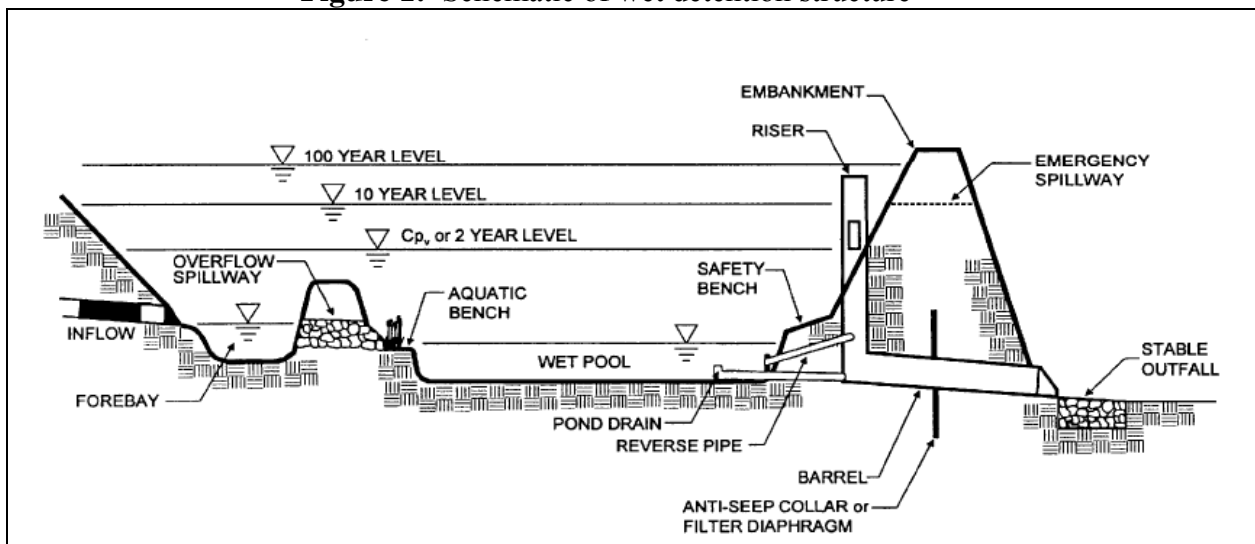
Figure 1: Schematic of wet detention structure
