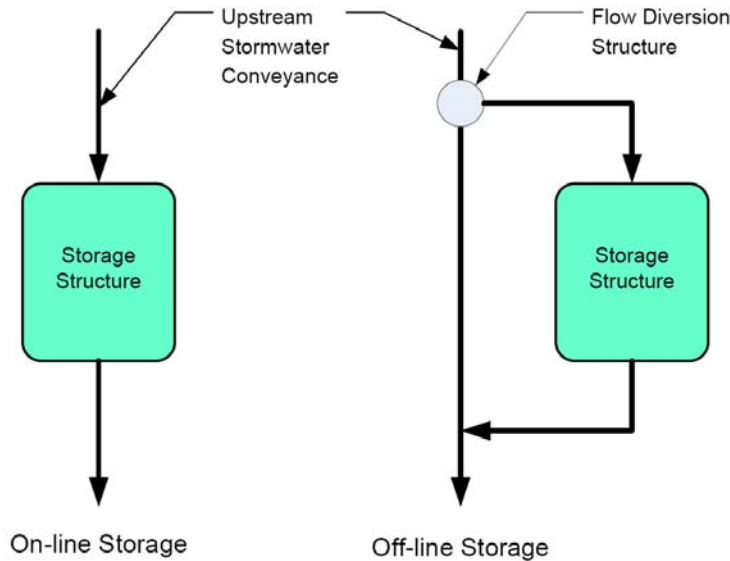
Figure 2: Online versus off-line storage
